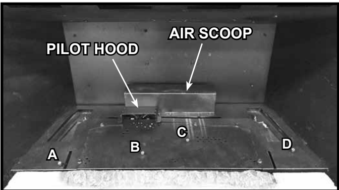
Figure 11 Empty Firebox with Front Hearth Installed
