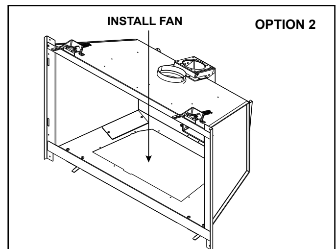
Figure 6.5 Through Valve Plate Opening (Option 2)
