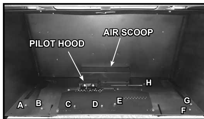
Figure 18. Empty Firebox with Front Hearth Installed
