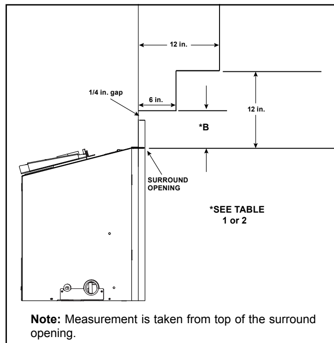
Figure 8.2 Minimum Vertical and Maximum Horizontal Dimensions- Non-Combustible
