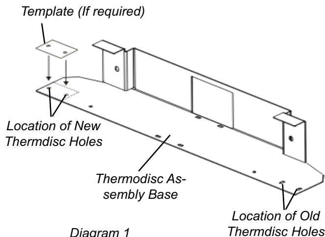
Thermodisc Assembly
